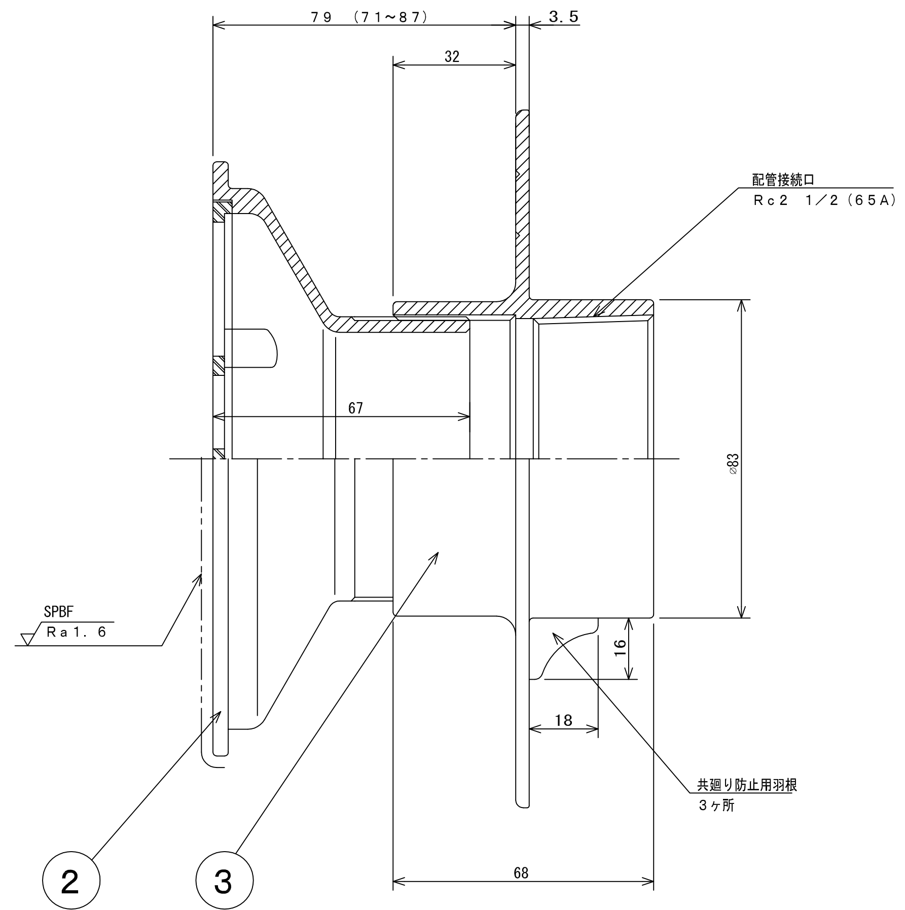
DL-CU65
